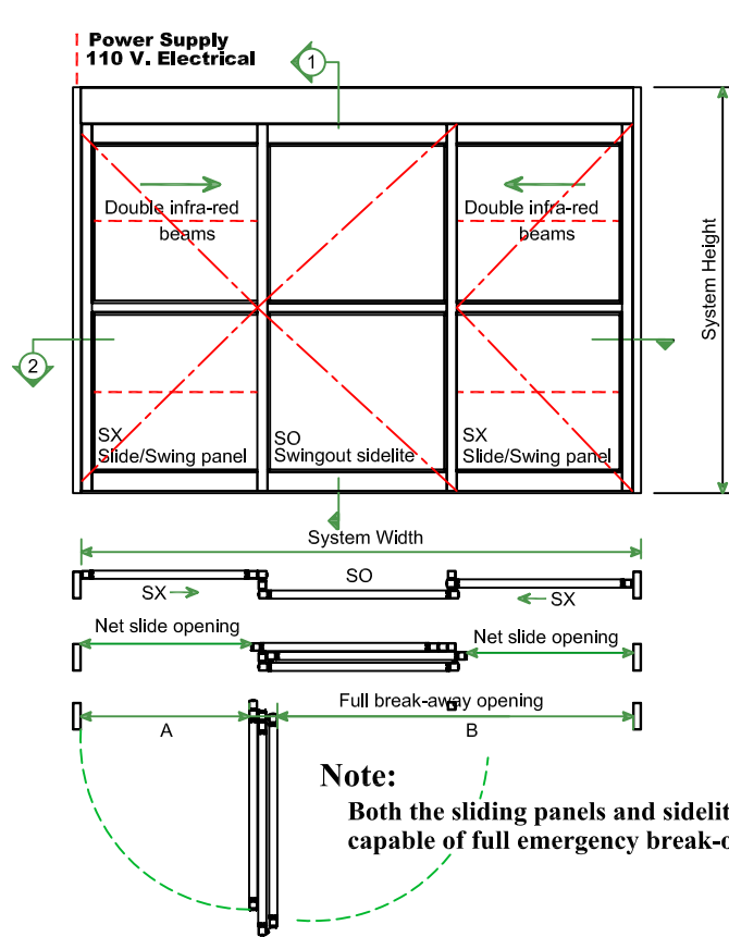
Elevation & floor plans Exterior view elevation
